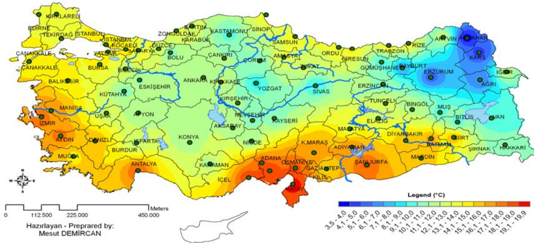
Figure 4 Annual mean temperatures of 78 stations (1971-2000).
