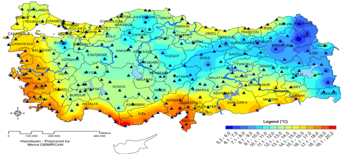
Figure 10 Distribution of extracted ERA40's values to Stations.
