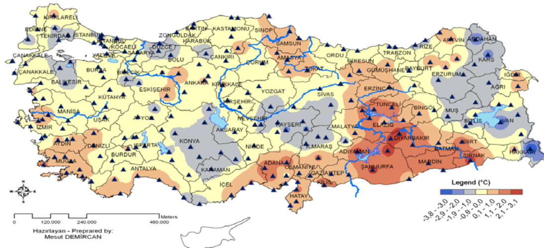
Figure 11 Distribution of errors between mean temperature of stations and mean temperature of ERA40.
